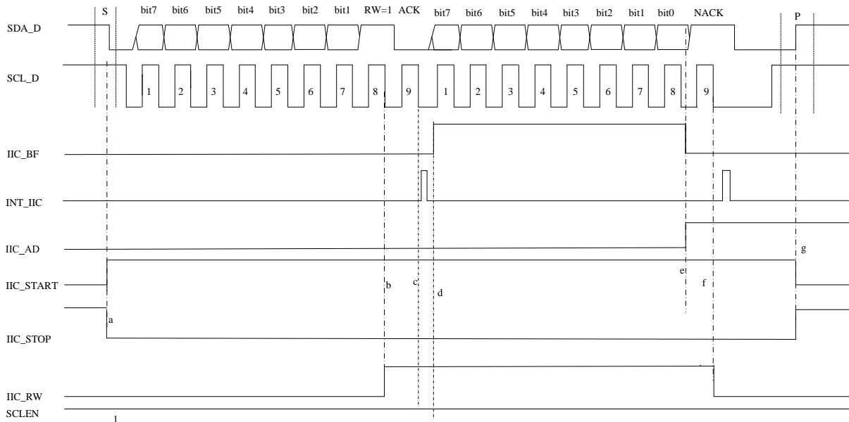
IIC master reading does not pull down the clock line diagram
