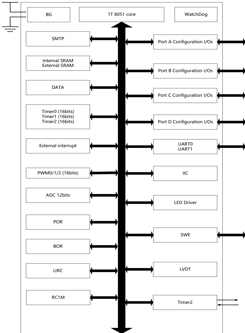
system architecture
