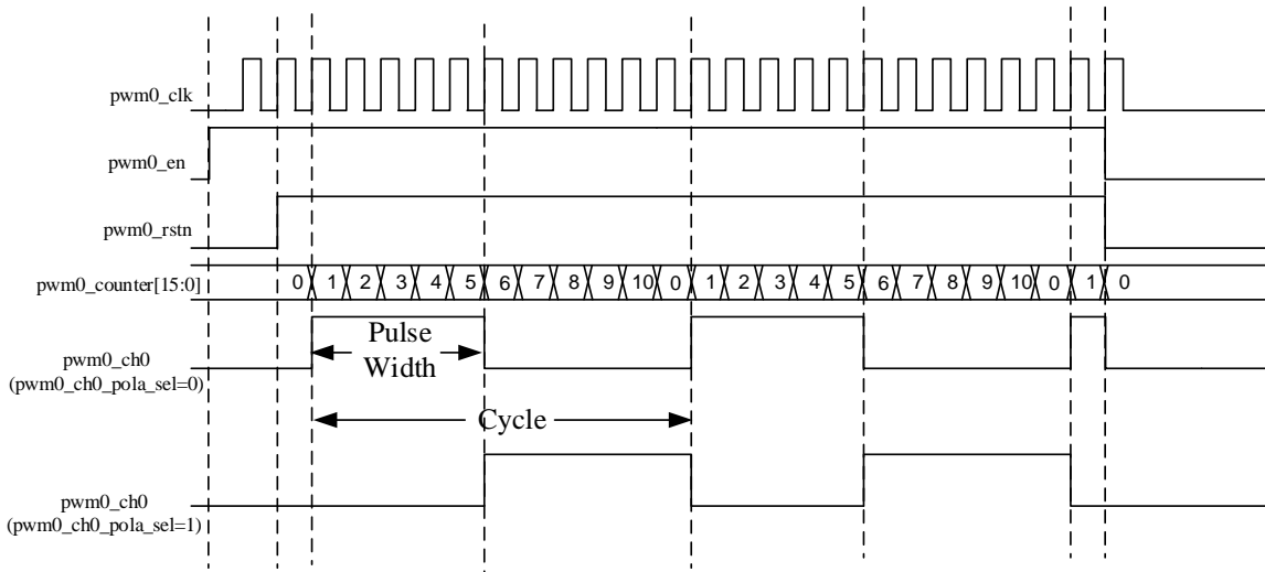
(PWM0_CH0_CNT=5. PWM0_MOD=10, duty_cycle=5/11)
