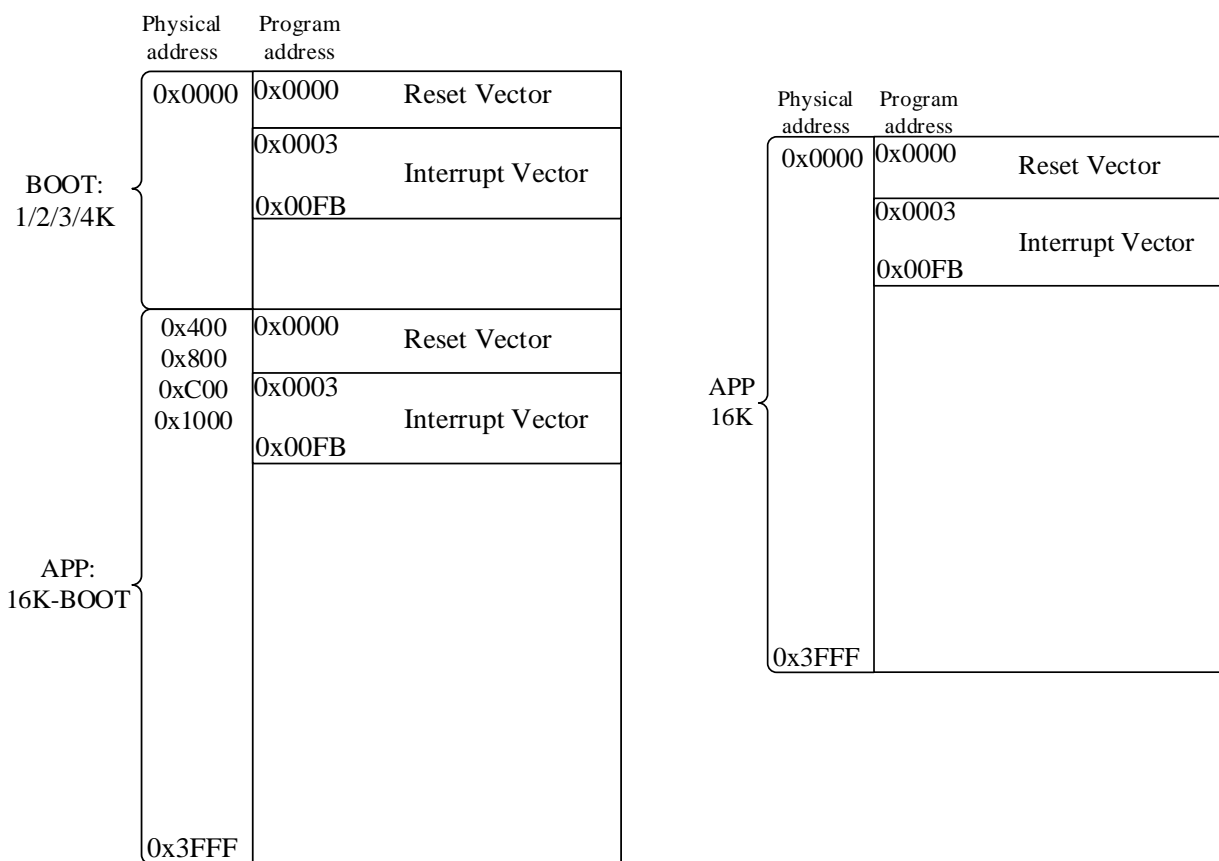
Left: BOOT and APP partition map; Right: APP map, not-BOOT map
