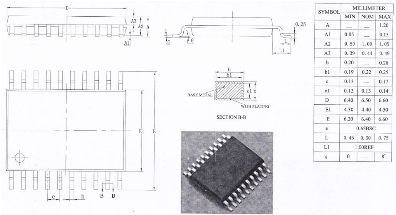
TSSOP20 package infographic
