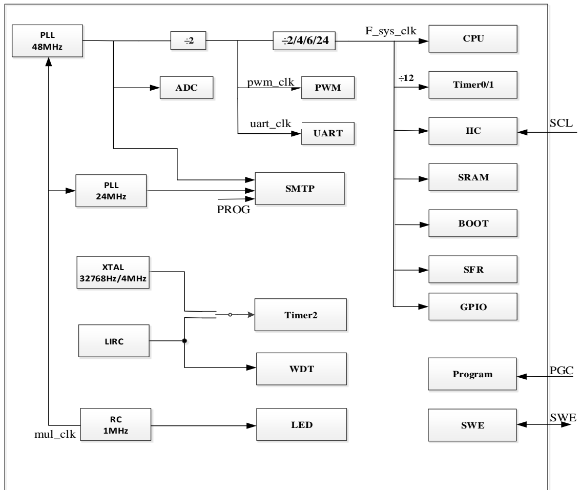
clock diagram
