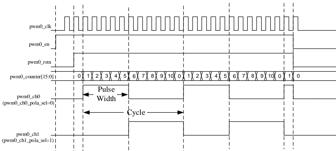
(PWM0_CH0, PWM0_CH1 complementary output)
