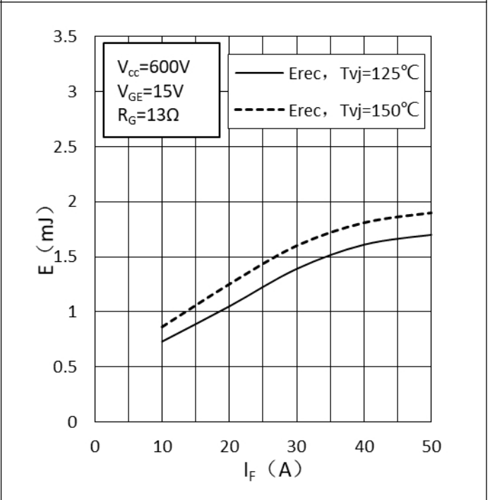
Fig.8 Typ. Switching Losses of Diode-Inverter
