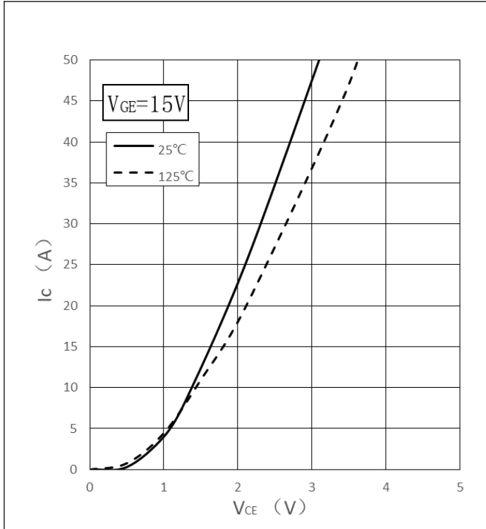
Fig.1 Typ. Output Characteristics-Inverter
