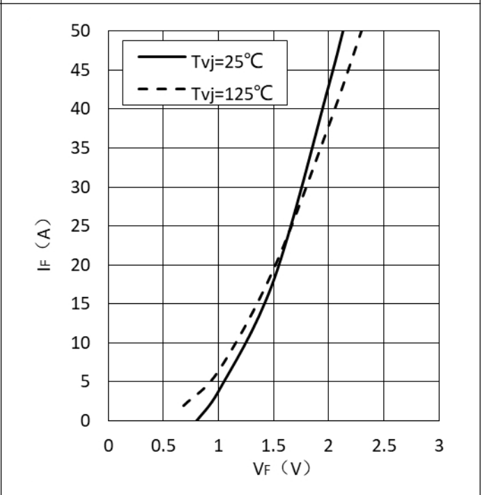
Fig. 12 Forward Characteristics of Diode- Brake-Chopper
