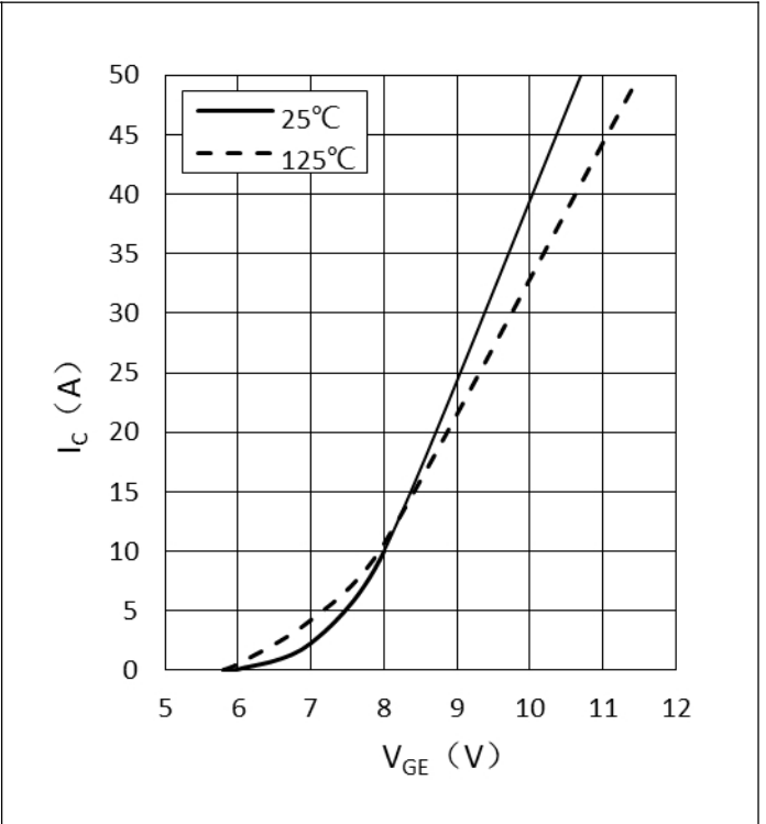
Fig.2 Typ. Transfer Characteristics-Inverter
