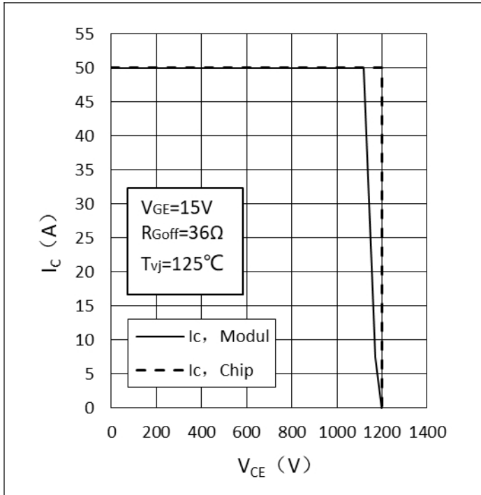
Fig.5 Reverse Bias Safe Operating Area (RBSOA) -Inverter
