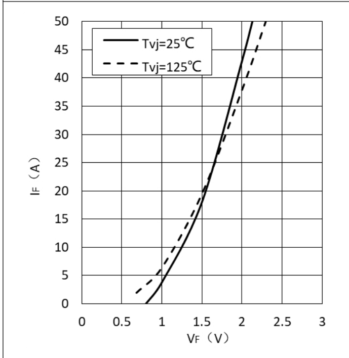
Fig.7 Typ. Forward Characteristics of Diode-Inverter
