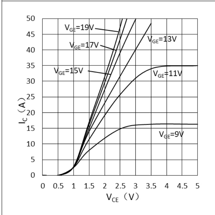
Fig.3 Typ. Output Characteristics-Inverter
