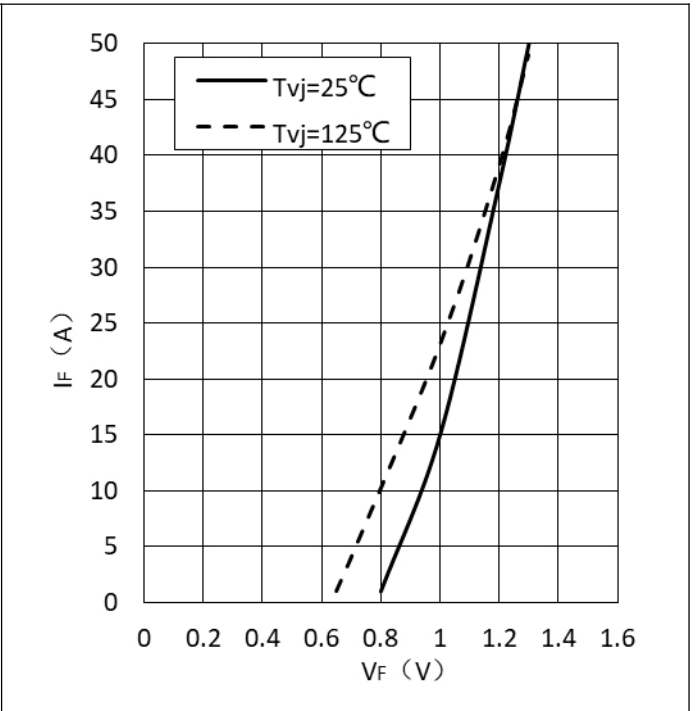
Fig.10 Forward Characteristics of Diode-Rectifier
