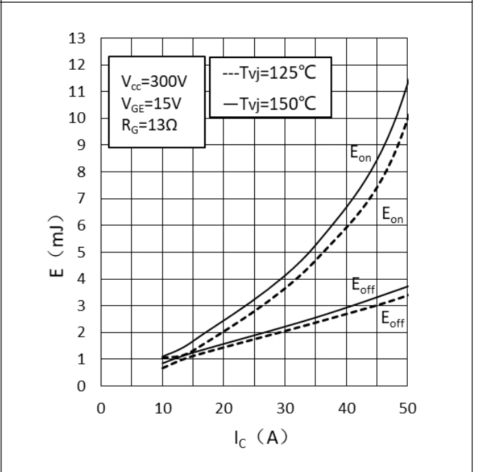
Fig.4 Switching Loss vs. Collector Current-Inverter
